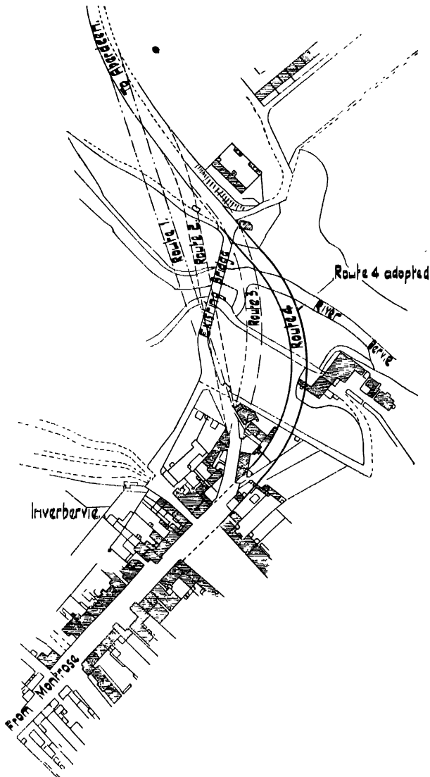
Fig. 11.—Study of Bridge Location from Ordnance Survey.
